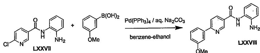
Scheme 15
